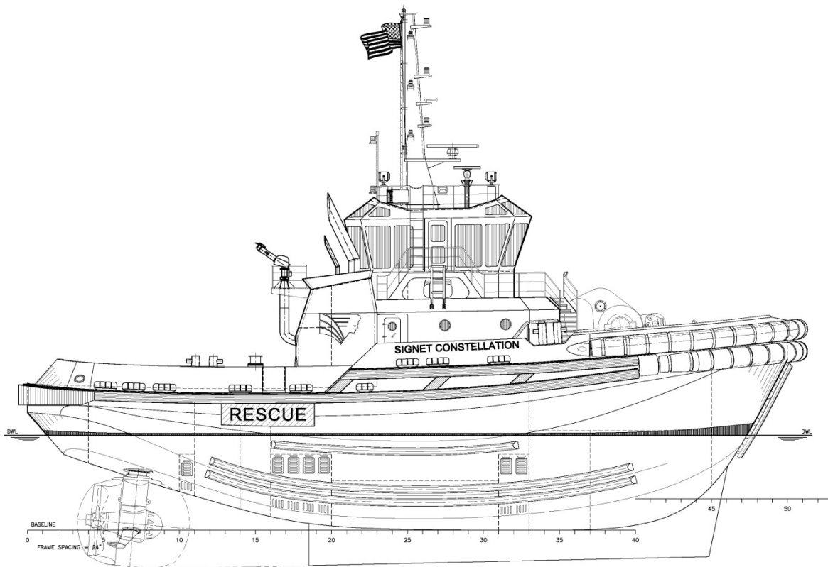
Profile View
