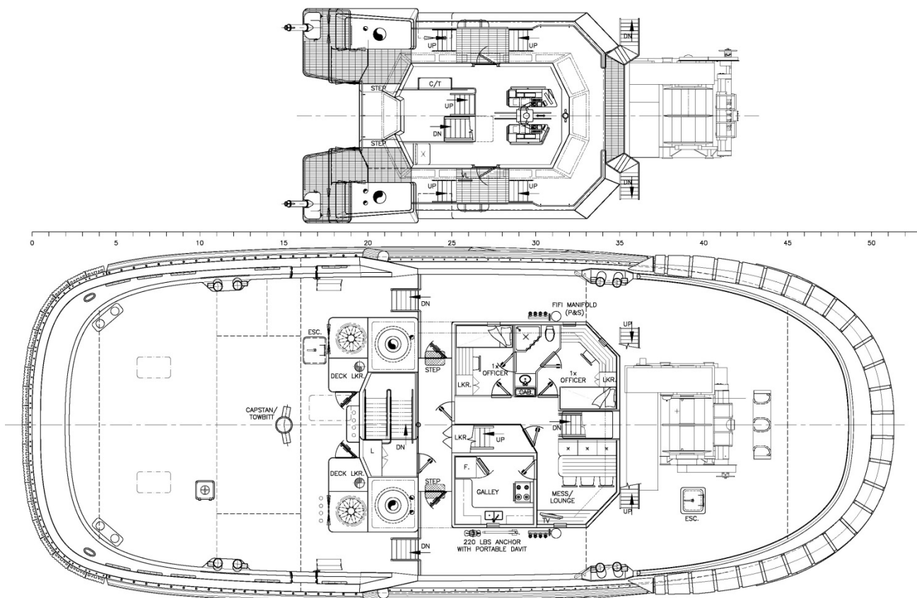
Plan View
