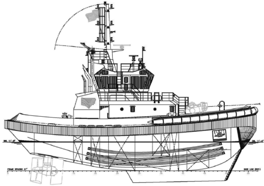
Profile View
